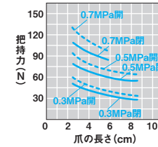
■CKA・CKB・CKD-20AS
