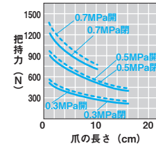
■CKA・CKB・CKD-50MS
